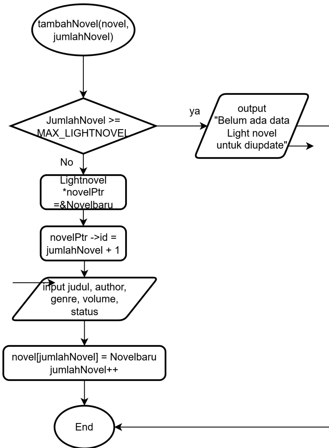
Gambar 1.5 Flowchart Create(tambahNovel)
